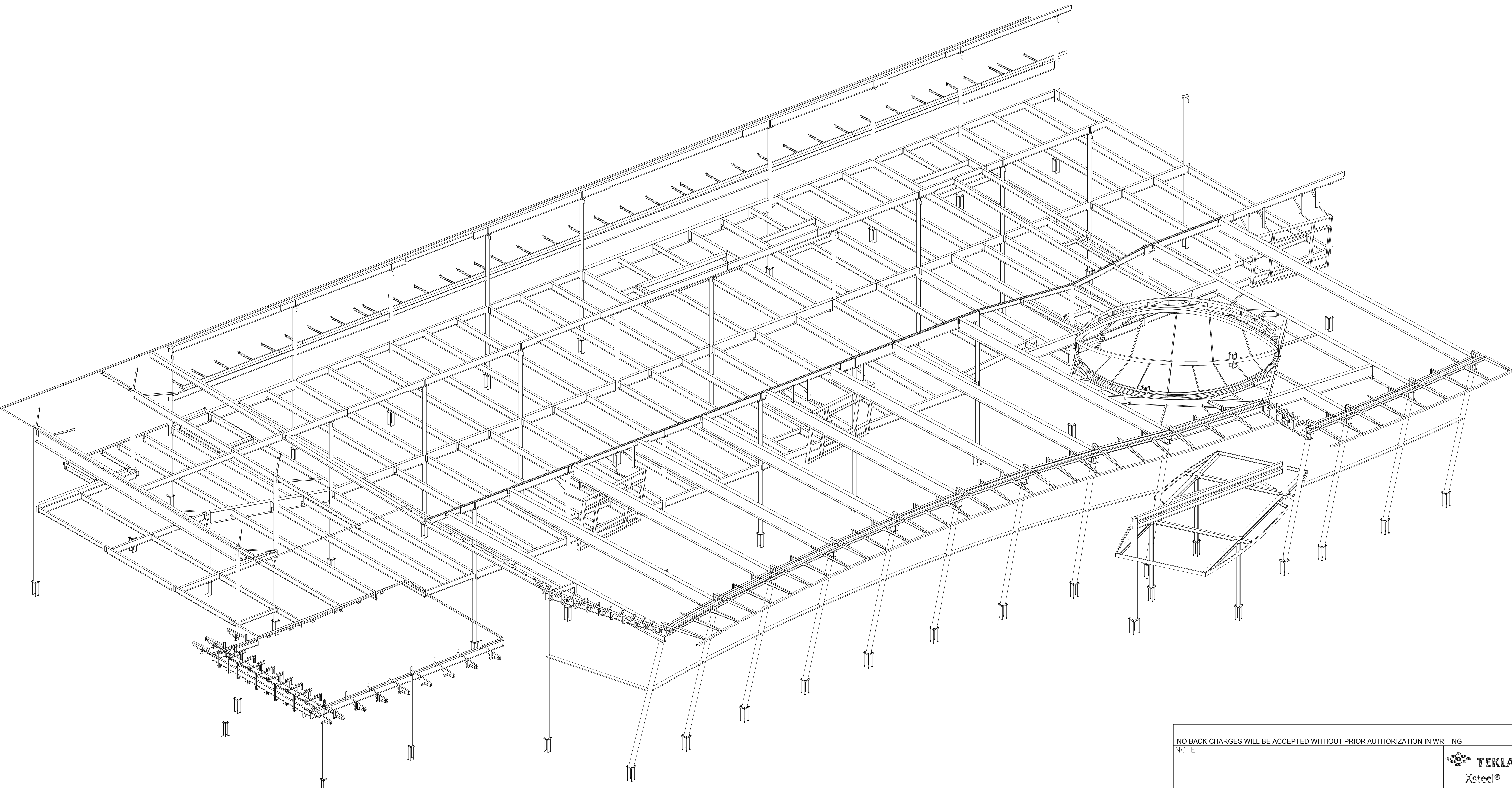
CLASSIC BMW PHASE 1 (PERSPECTIVE VIEW) 182 TONNES
