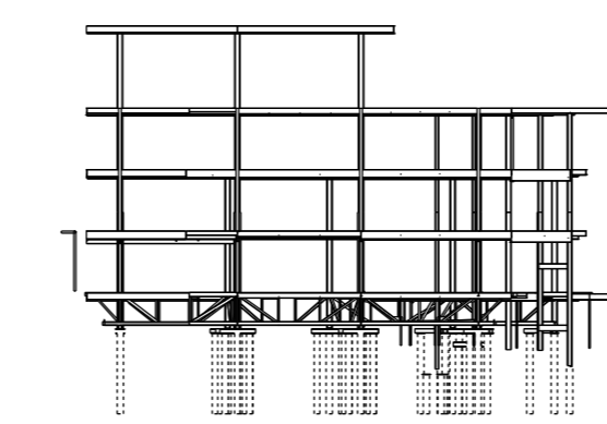
EAST ELEV.
