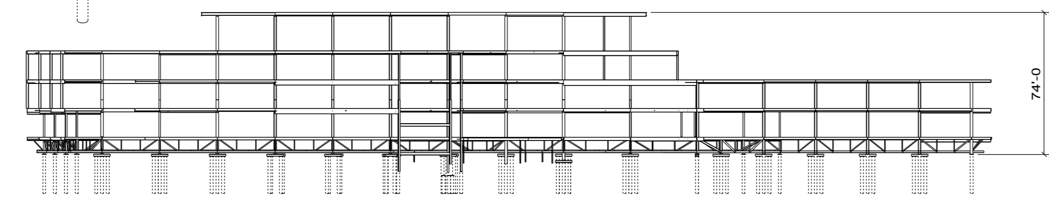
SOUTH ELEV.
