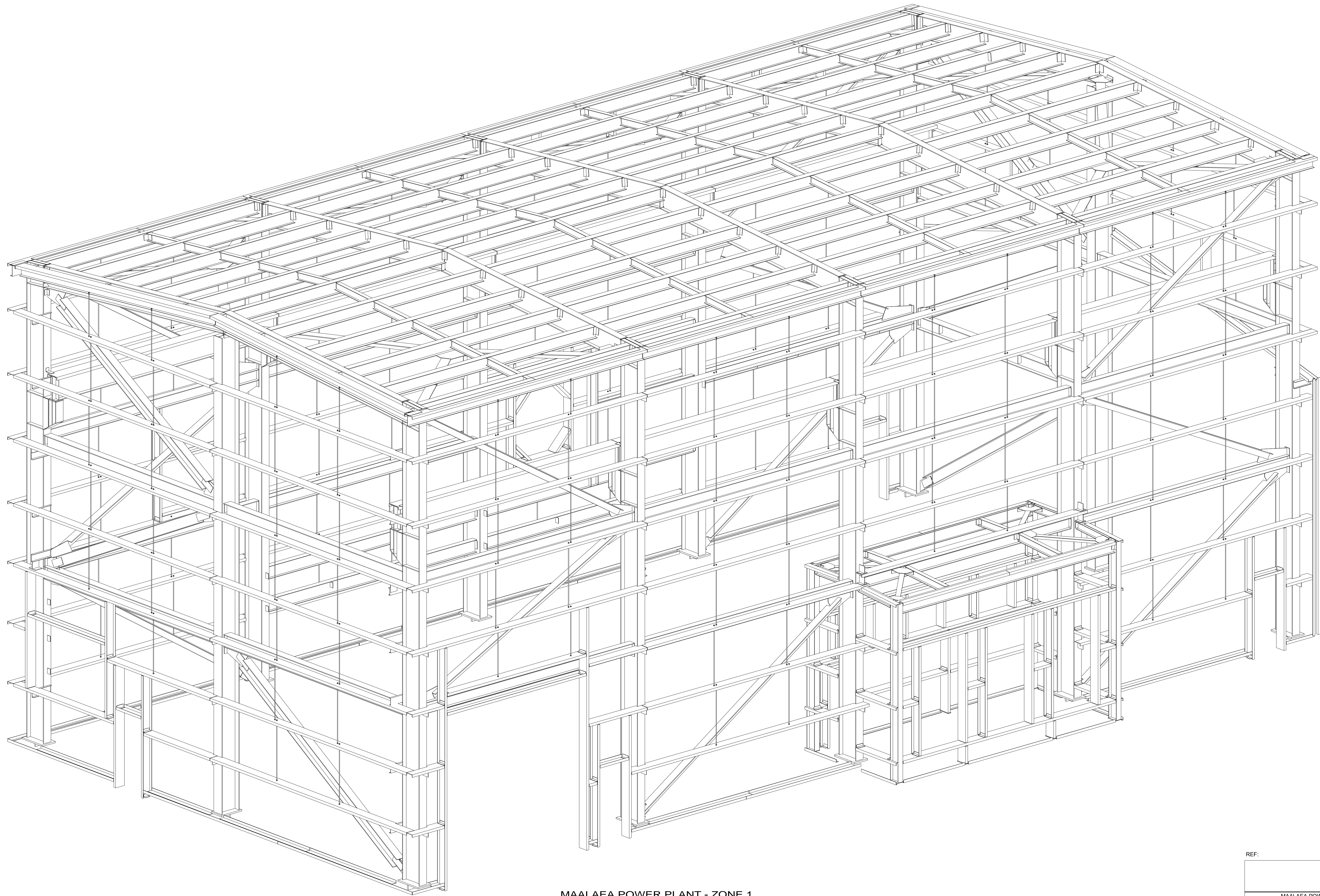
MAALAEA POWER PLANT - ZONE 1 (PERSPECTIVE VIEW) 140 TONNES
